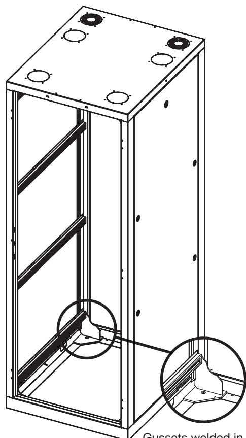
Gussets welded in place to add strength required for Z4, 8 places per frame
